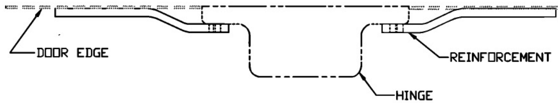
LEFT REINFORCEMENT TOP VIEW
