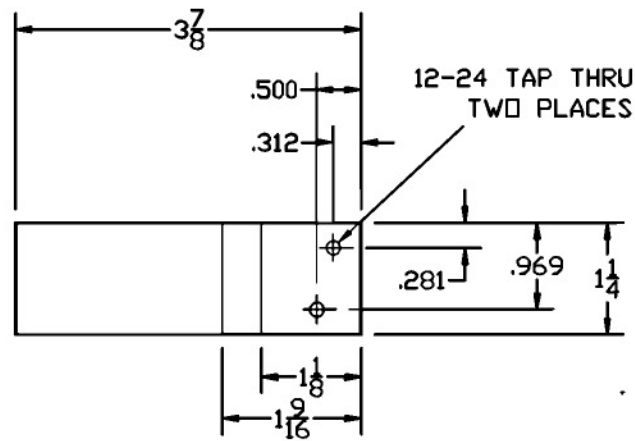
LEFT REINFORCEMENT TOP VIEW
