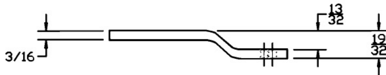
LEFT REINFORCEMENT SIDE VIEW
